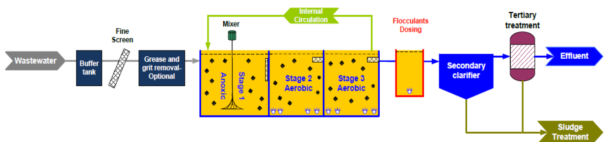
Figure 3 WWTP schematic (Aquis 2015)
